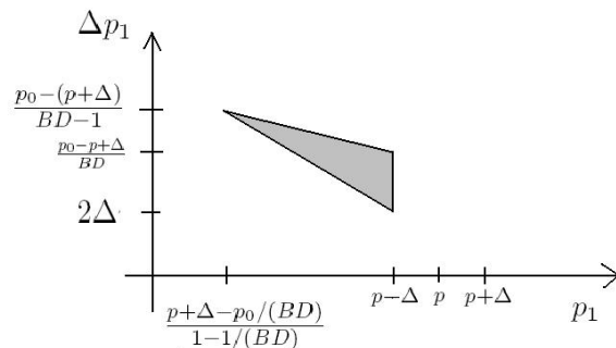
Figure A.11: The area S_1(\Delta, p) is colored grey.
