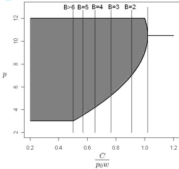
Figure 6: The upper curve represents p_{Z_{max}} according to \frac{C}{p_0w} . The lower curve represents p_{Z_{min}} according to \frac{C}{p_0w} . The area which is colored grey represents the values of the initial price for which a cooperative of myopic agents is viable. When k = N/B maximizing agents are included in the mixture, the area of initial price for which the mixture is viable is reduced to the left side of the vertical lines. p_0 = 12 , \bar{\alpha} = 2 and from (43), the position of the vertical lines is defined by \frac{C}{p_0w} = \frac{(1+A)^2}{A} \frac{B}{(1+B)^2} when B \leq \bar{\alpha}(\bar{\alpha} + 1) = 6 and by \frac{C}{p_0w} = \frac{1}{\bar{\alpha}} when B > \bar{\alpha}(\bar{\alpha} + 1) = 6 .
